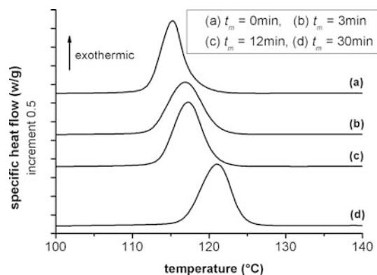
Fig. 4 DSC cooling curves of iPP samples, after cryogenic MM for different t_m . The cooling rate was 5 °C/min
