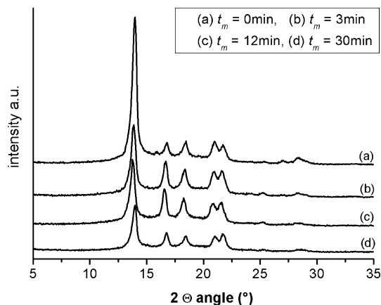
Fig. 3 X-ray diffraction patterns of compression molded iPP samples, after cryogenic MM for different milling times t_m
